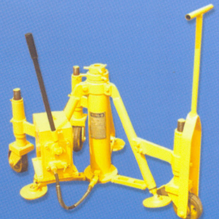
CAPACITY : 5 T , LIFT : 915 MM , CLOSED HT : 660 MM
