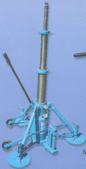
MODEL:VTEJ-3/575 CAPACITY : 3 T LIFT : 575 MM CLOSED HT:325 NO.OF STAGES:3
